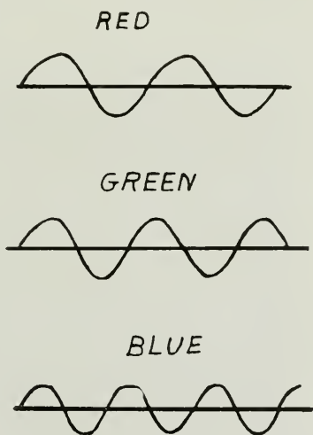
Fig. 8. Relative Wave Lengths of Red, Green and Blue.
